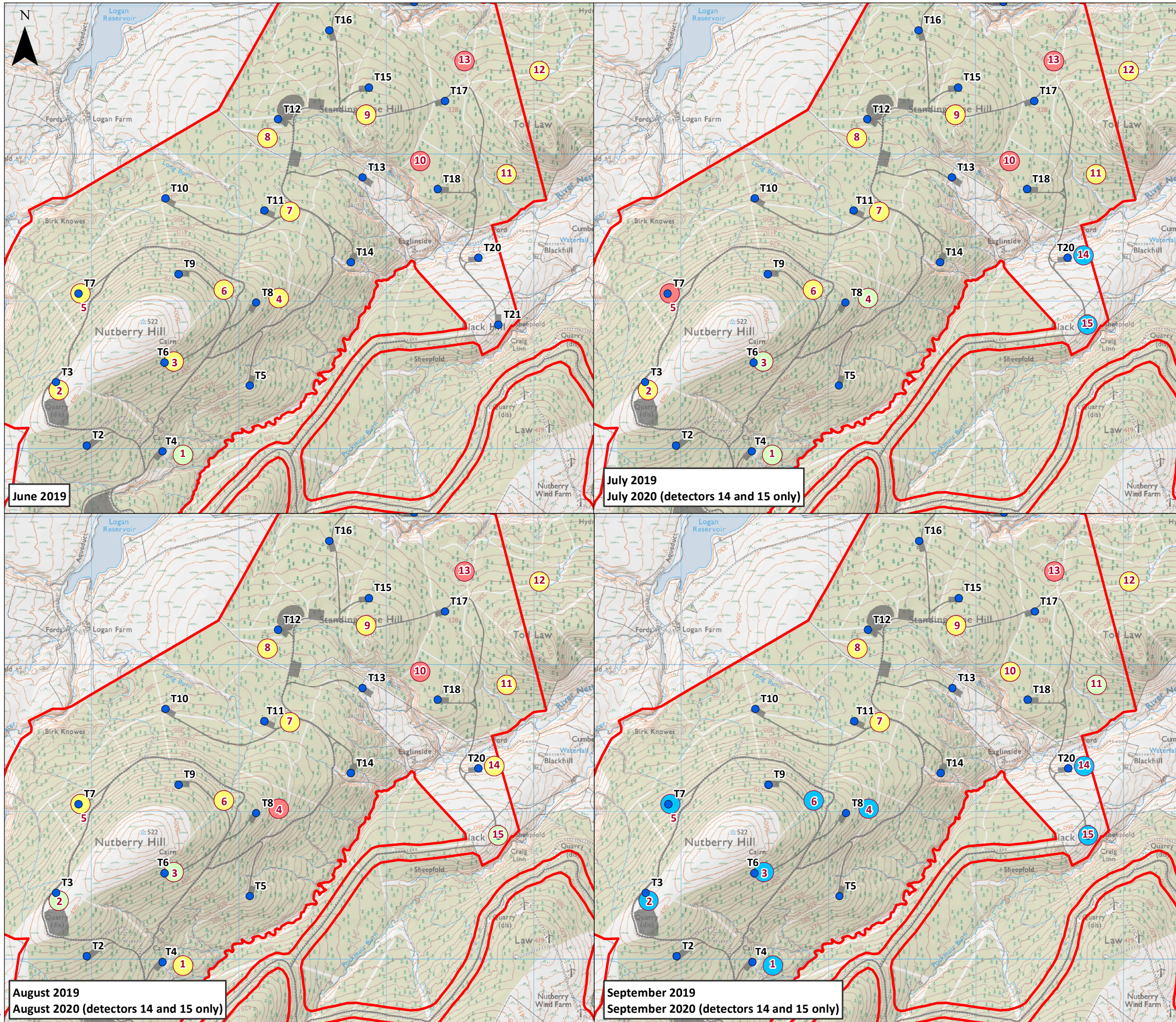
Cumberhead West Wind Farm Environmental Impact Assessment Report Figure 7.10 Overall Median Risk Assessment (June, July & August and September) for Soprano Pipistrelle
